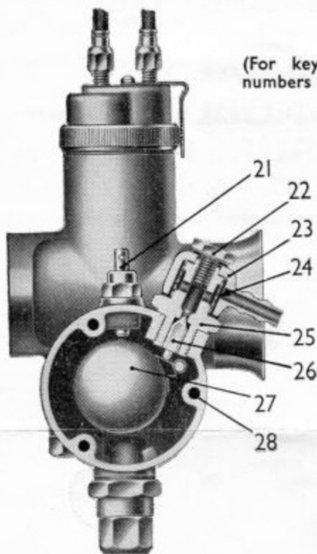
Fig. 1—Section through float chamber.
